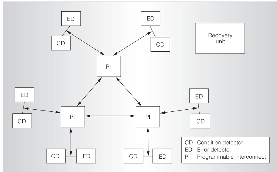
Figure 2. Distributed design of our programmable error-patching hardware.
